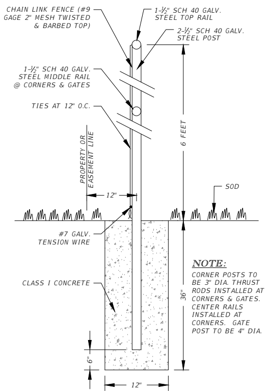
SUB-DETAIL D
