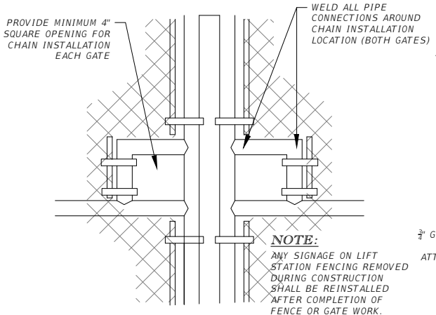
SUB-DETAIL G (GATE LATCH)
