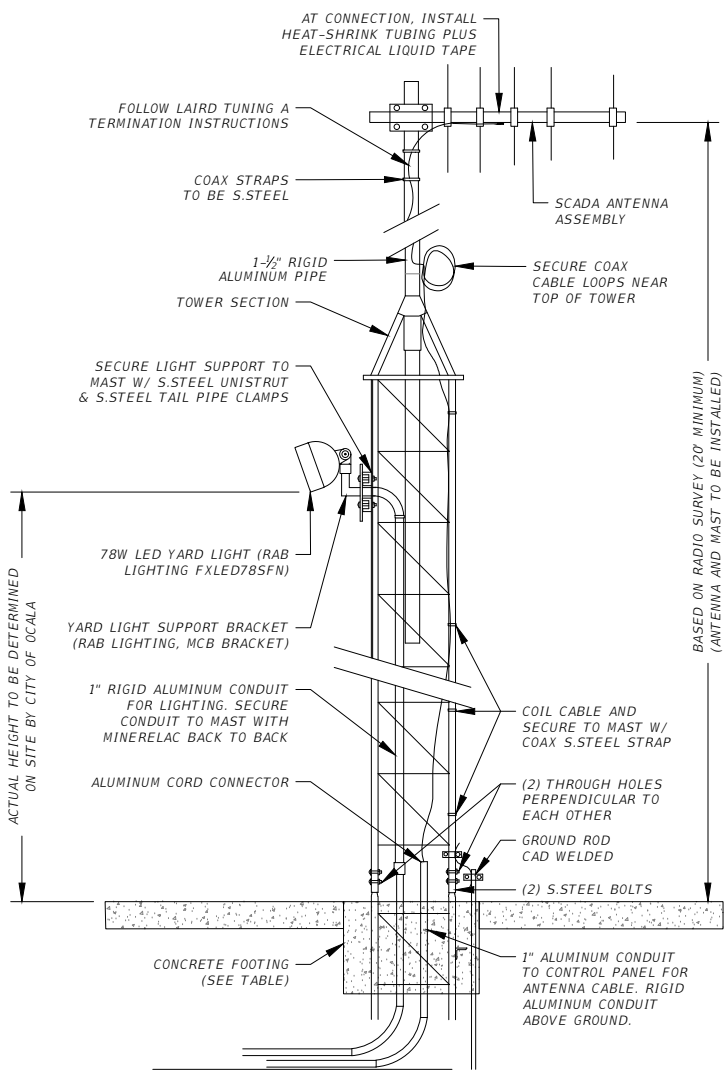
SUB-DETAIL C
