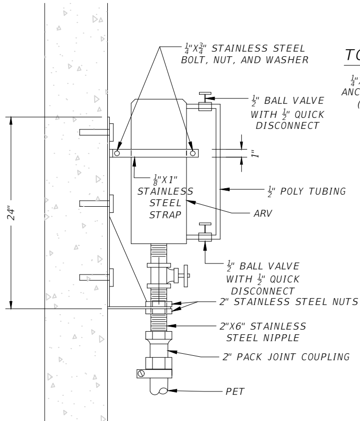
SIDE VIEW
