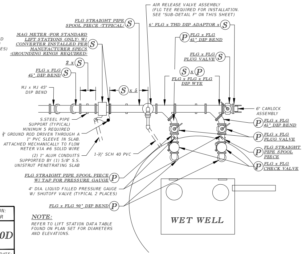
SUB-DETAIL E
