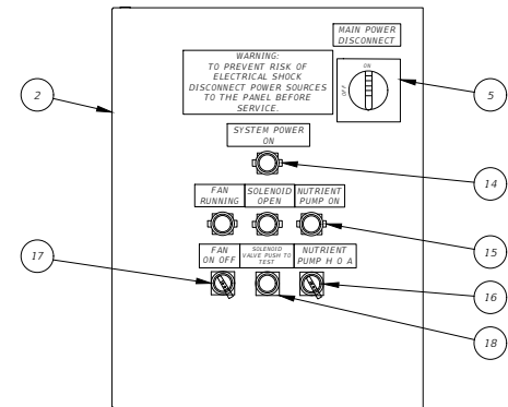
ELECTRICAL CONTROL PANEL SWING OUT PANEL LAYOUT
