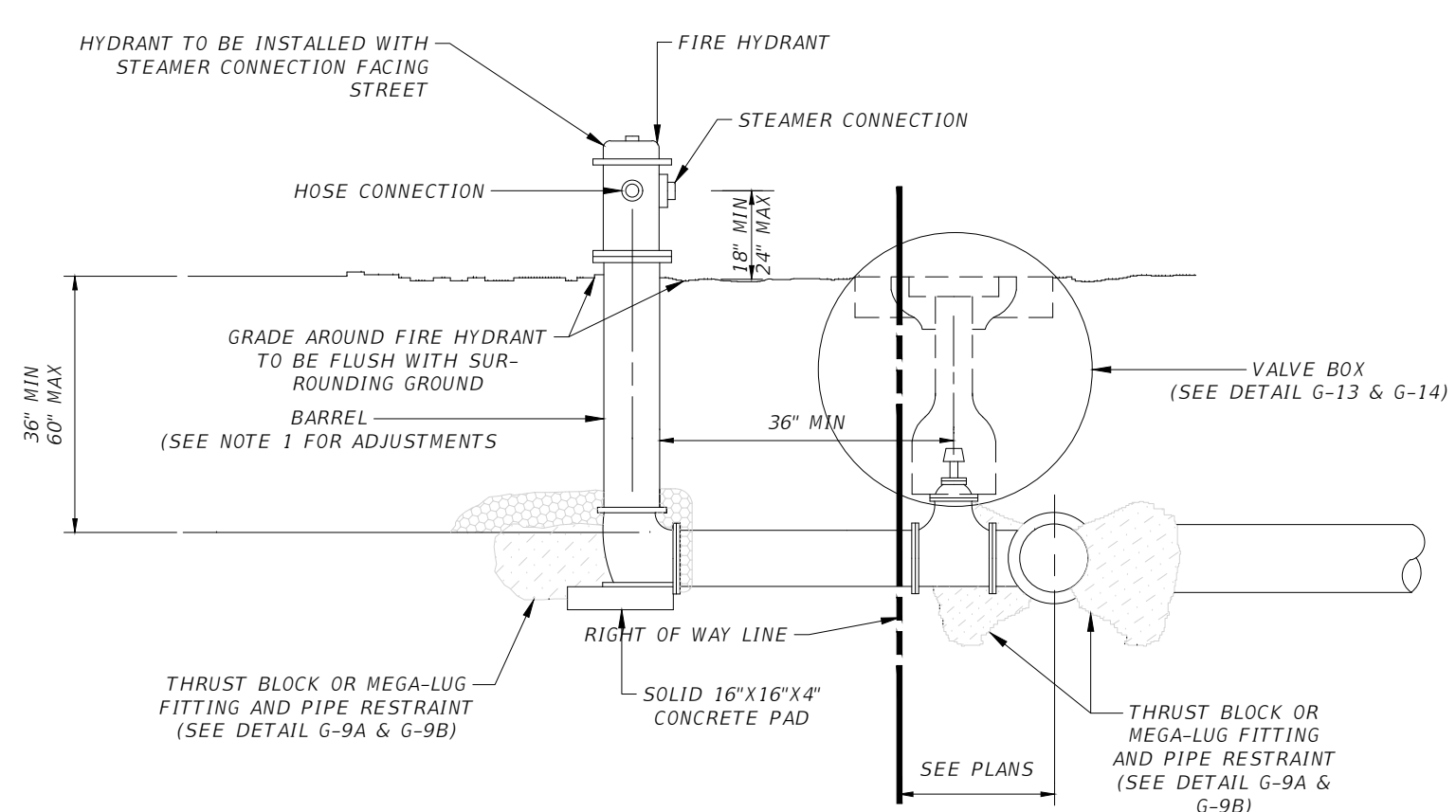
SECTION VIEW
