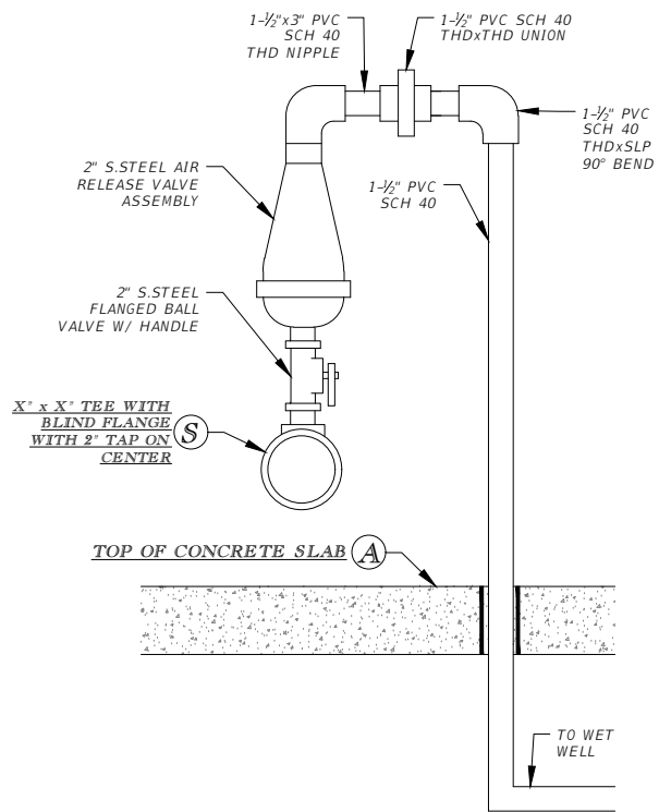
SUB-DETAIL F
