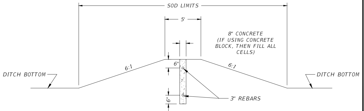
SIDE VIEW
