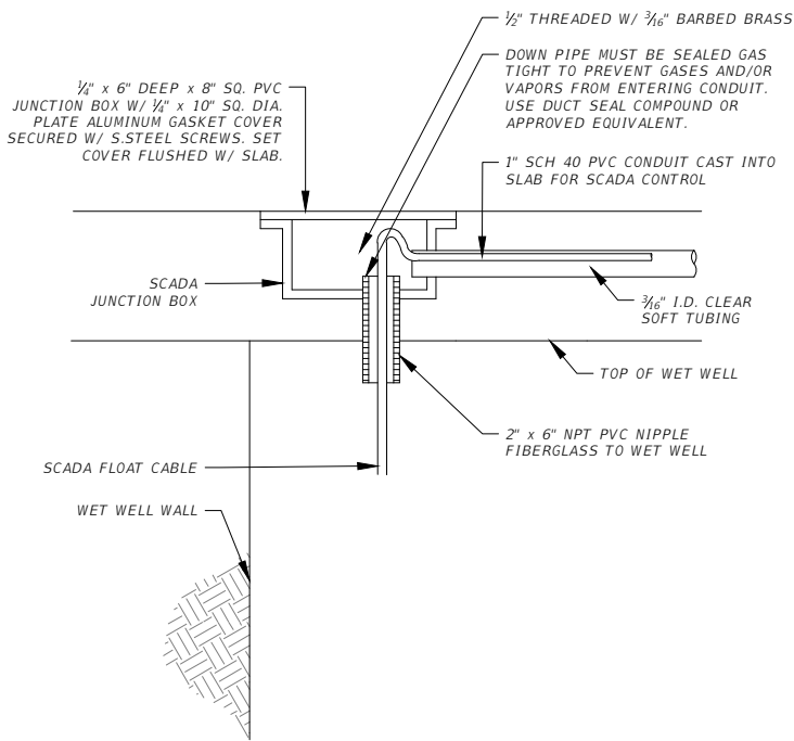
SUB-DETAIL A
