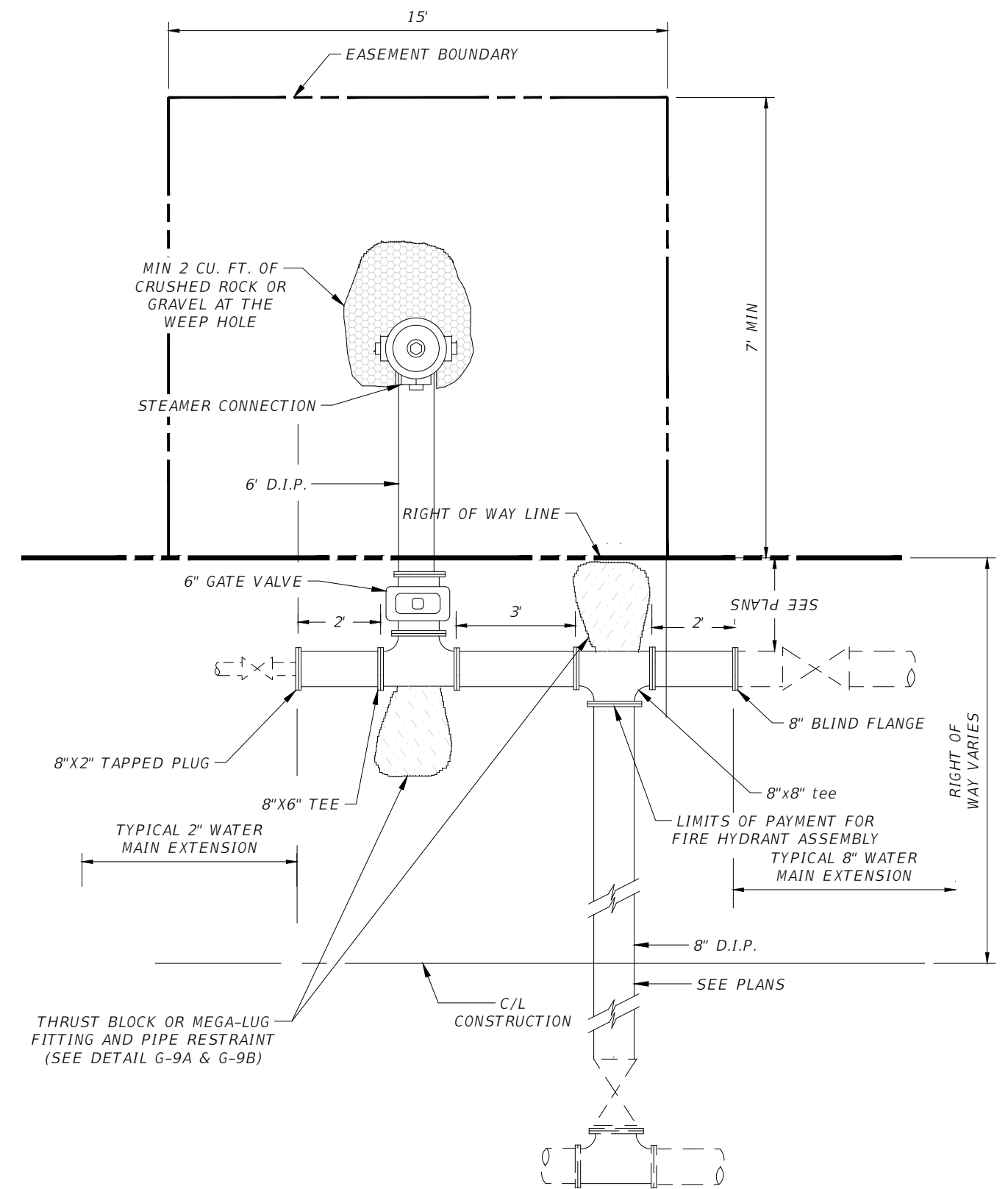
PLAN VIEW
